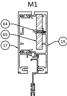
REINFORCED MULLION - CAPTURE
