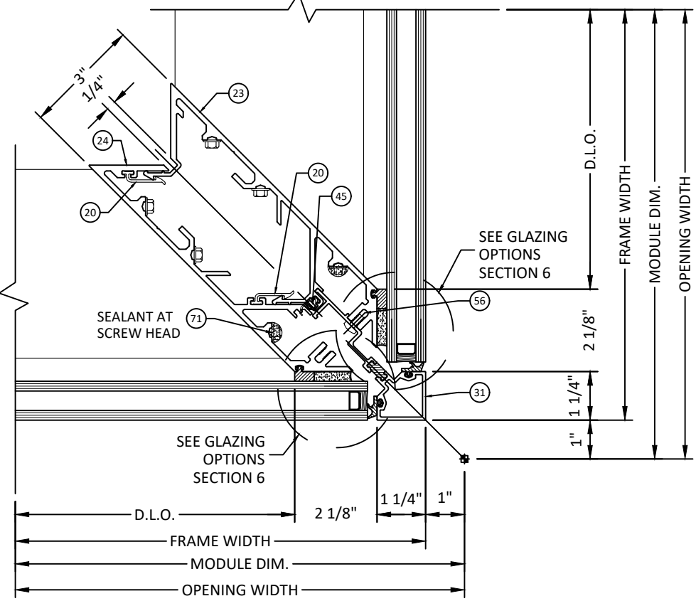
5 4.2 HORIZONTAL SECTION OUTSIDE CORNER - SSG
