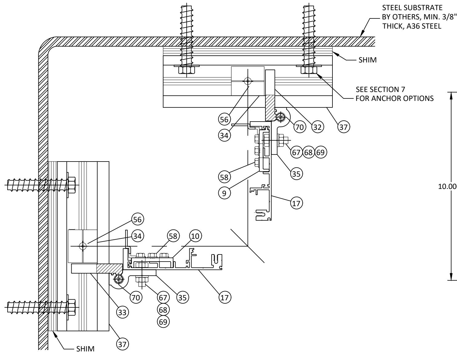
21 8.4 HORIZONTAL SECTION INSIDE CORNER
