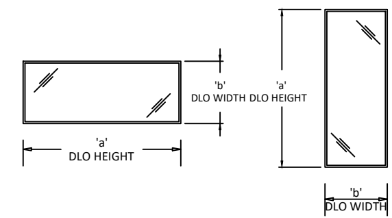
PANEL DIMENSIONS ( 'a' ≥ 'b' )
