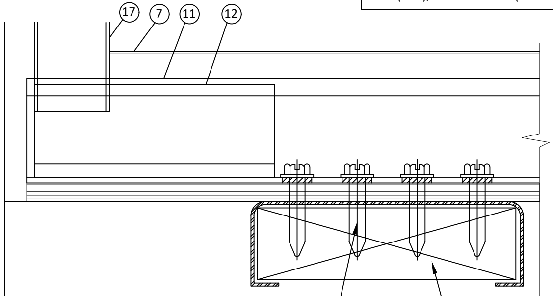
EXTERIOR VIEW JAMB-ANCHOR (TYPICAL) SEE NOTES 1-3 WOOD OR STEEL STUD SUBSTRATE BY OTHERS. SEE INSTALLATION ANCHOR REQUIREMENTS
