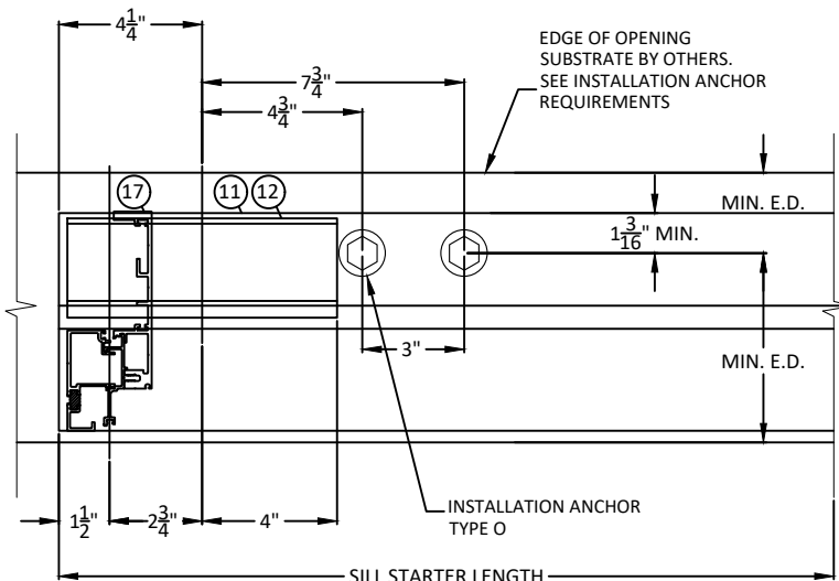
9 HORIZONTAL SECTION 7.3 SILL STARTER AT JAMB CONFIG 2
