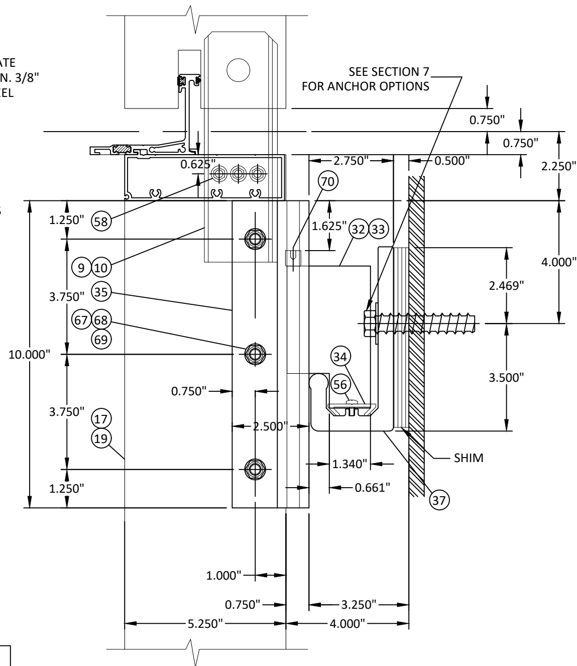
VERTICAL SECTION ANCHOR AT STEEL SUBSTRATE
