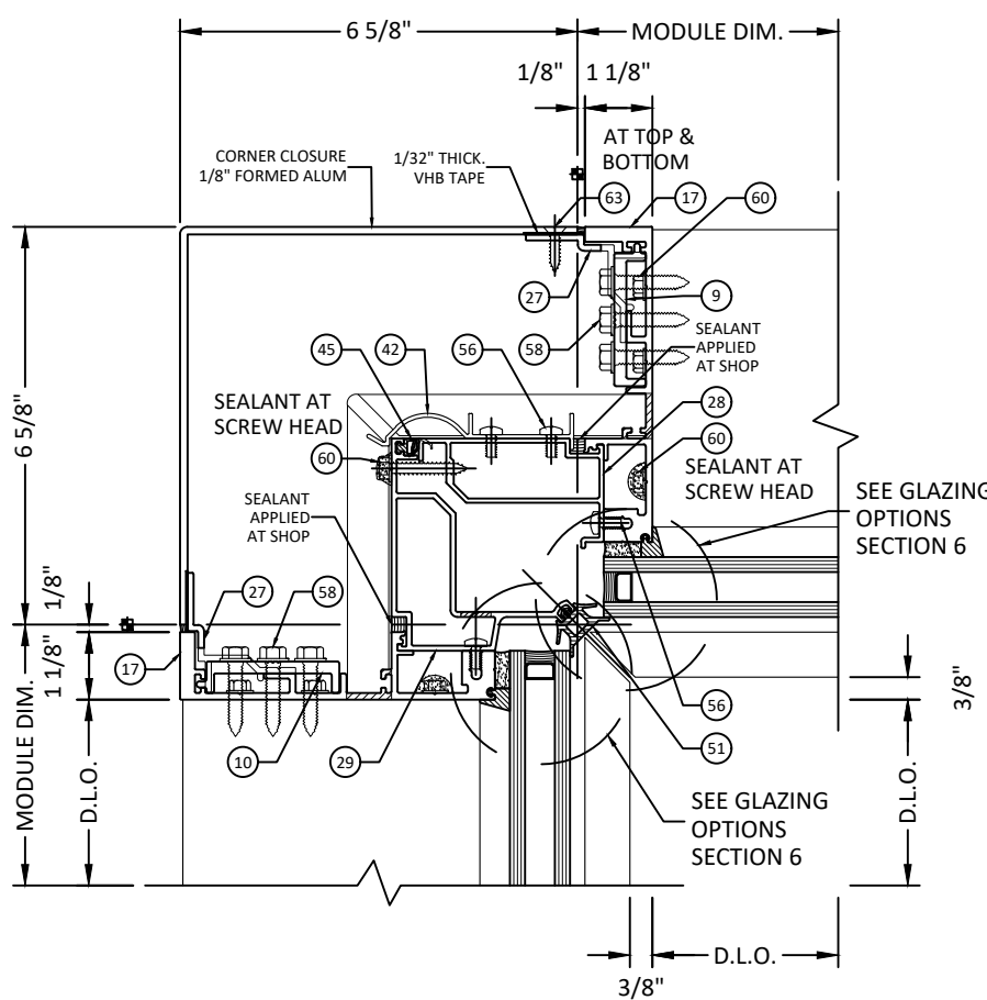
2 4.2 HORIZONTAL SECTION INSIDE CORNER - SPLICE - CAPTURE/SSG
