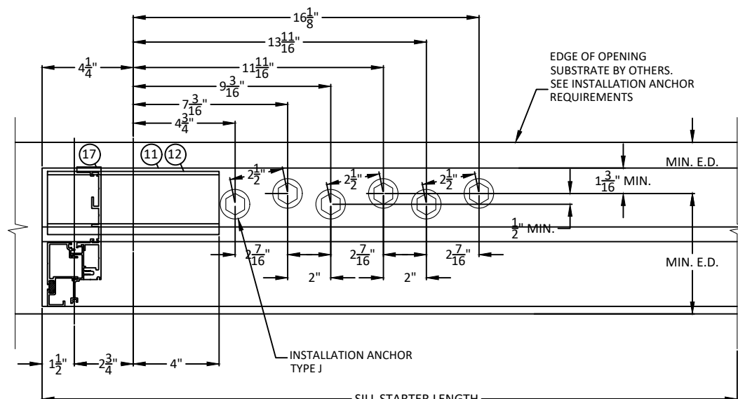
7 HORIZONTAL SECTION 7.3 SILL STARTER AT JAMB CONFIG 2
