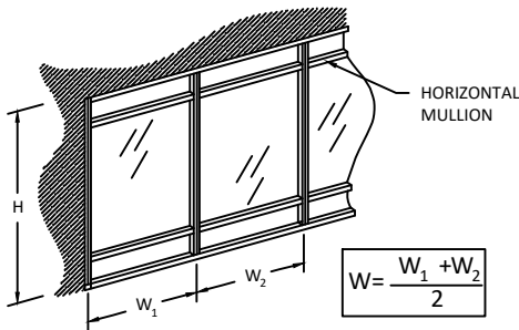
SINGLE SPAN
