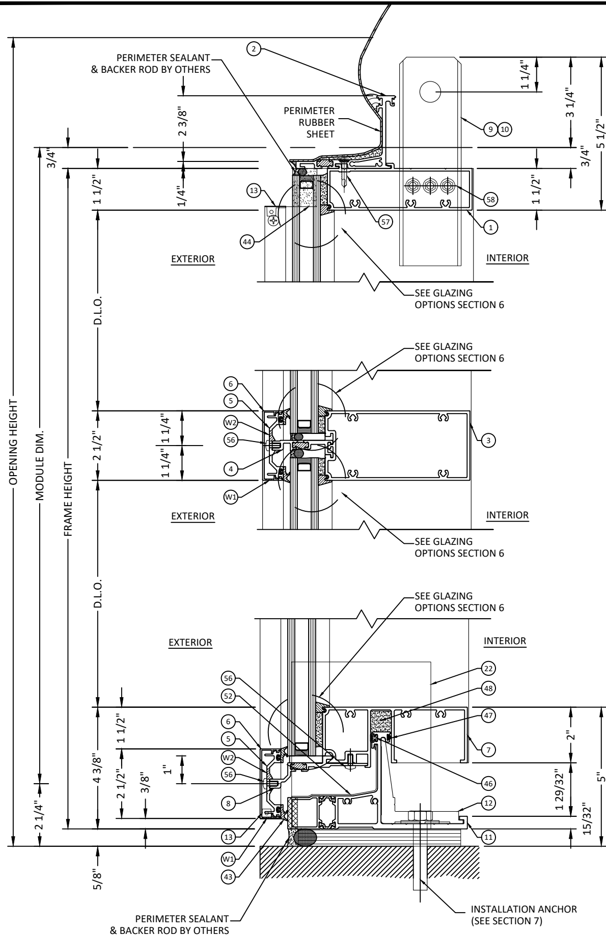
1 3.0 VERTICAL SECTION CAPTURE
