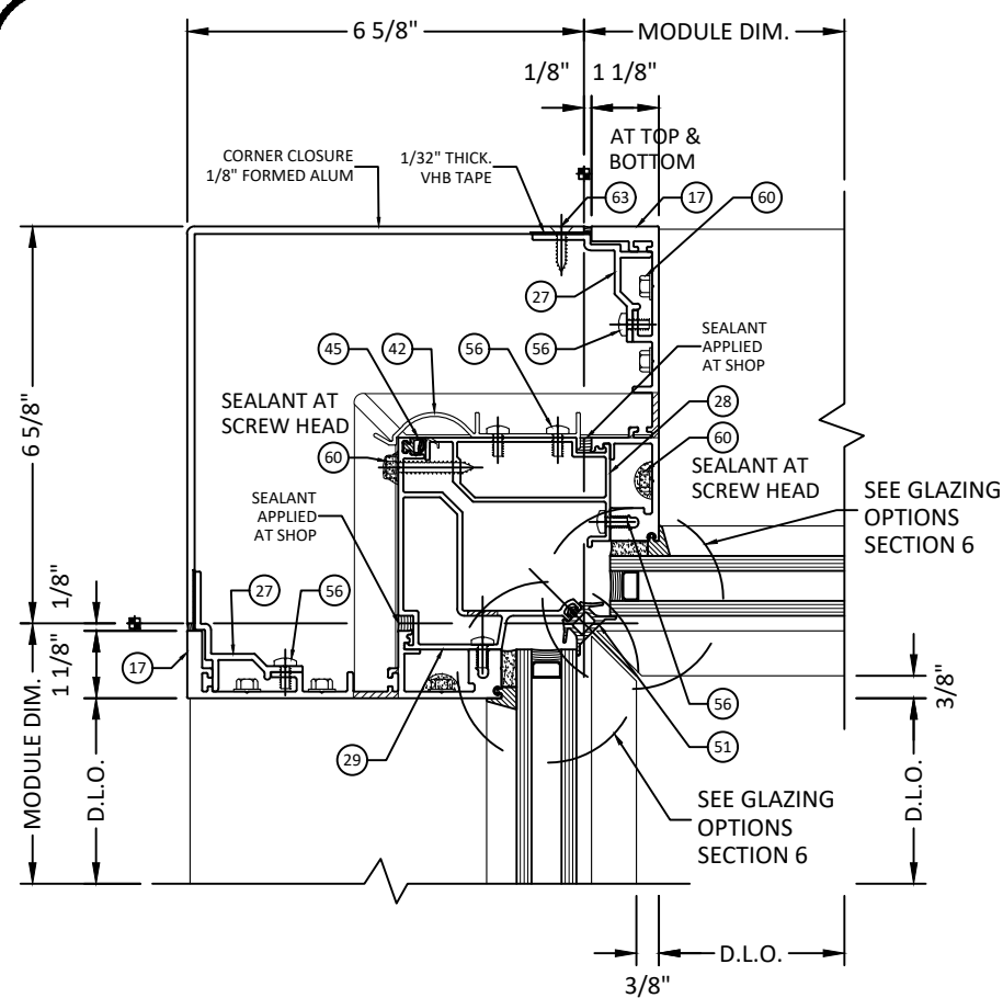
1 4.2 HORIZONTAL SECTION INSIDE CORNER - CAPTURE/SSG
