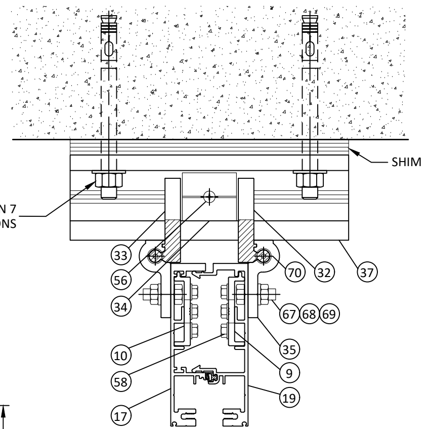
19 8.2 HORIZONTAL SECTION AT VERTICAL MULLION
