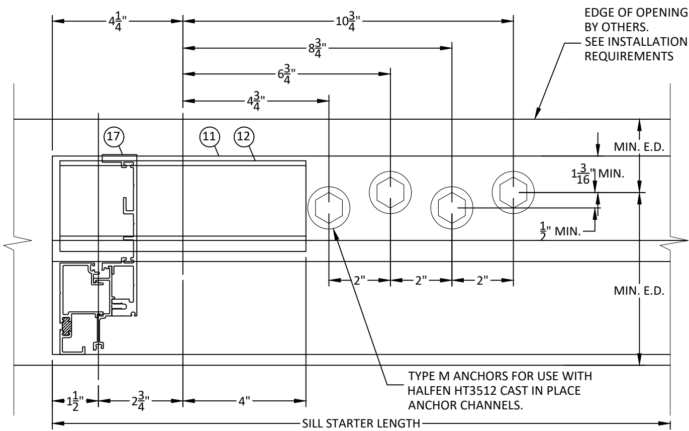
3 HORIZONTAL SECTION 7.2 SILL STARTER AT JAMB CONFIG 1
