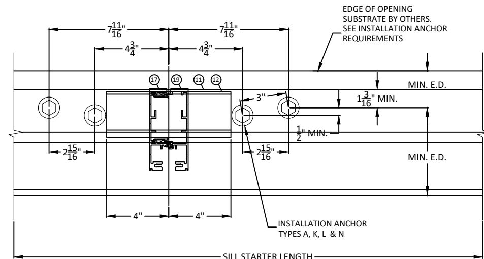
6 HORIZONTAL SECTION 7.3 SILL STATER AT MULLION CONFIG 2
