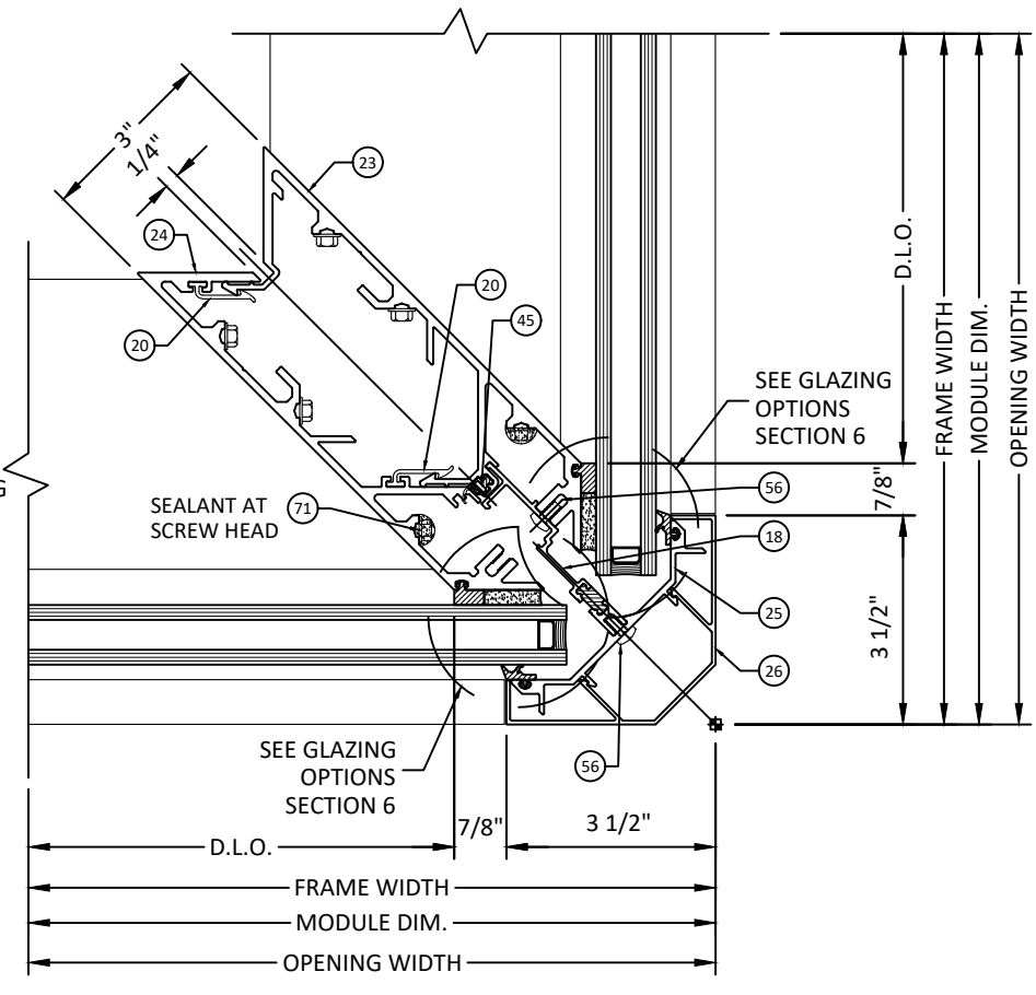
3 4.2 HORIZONTAL SECTION OUTSIDE CORNER - CAPTURE
