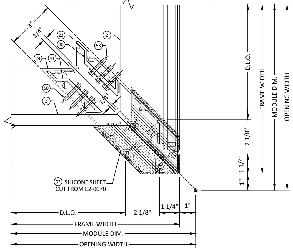
4 4.2 HORIZONTAL SECTION OUTSIDE CORNER - SPLICE - SSG
