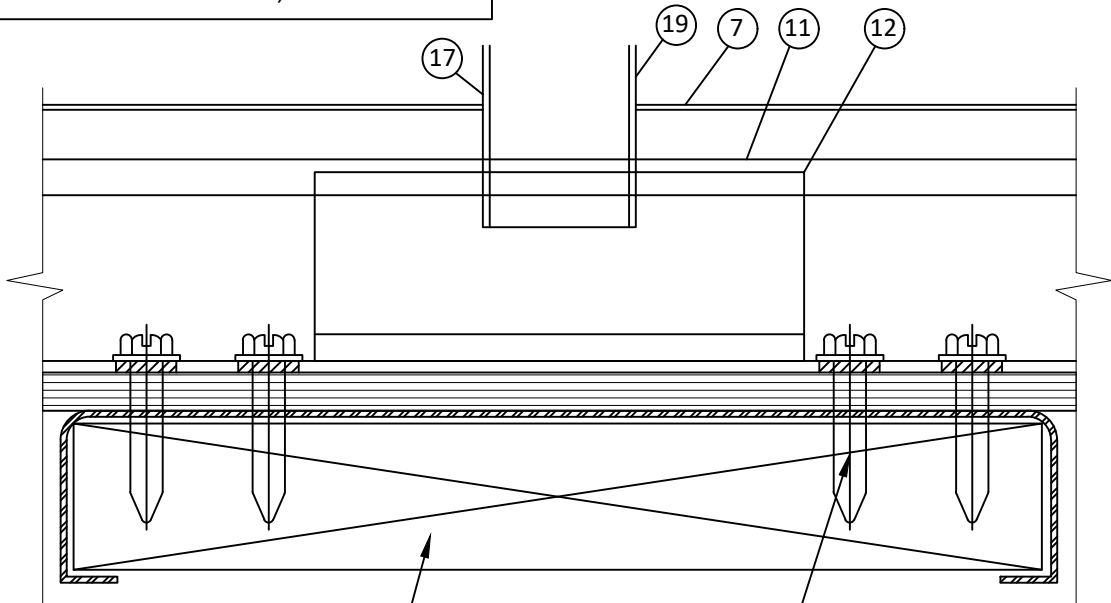
EXTERIOR VIEW MULLION-ANCHOR (TYPICAL) SEE NOTES 1-3 WOOD OR STEEL STUD SUBSTRATE BY OTHERS. SEE INSTALLATION ANCHOR REQUIREMENTS
