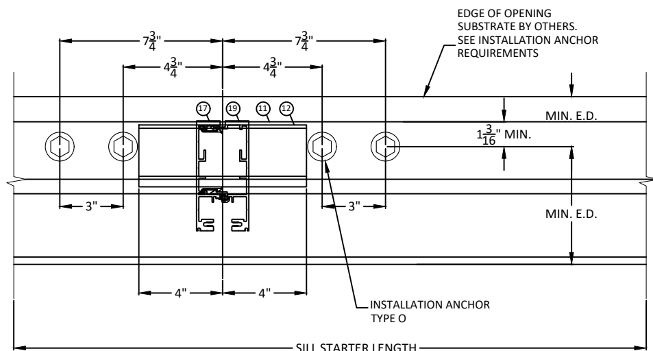
20 HORIZONTAL SECTION 7.3 SILL STATER AT MULLION CONFIG 2
