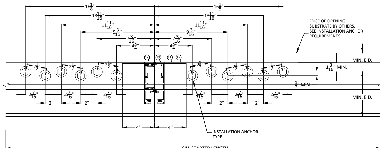
8 HORIZONTAL SECTION 7.3 SILL STATER AT MULLION CONFIG 2
