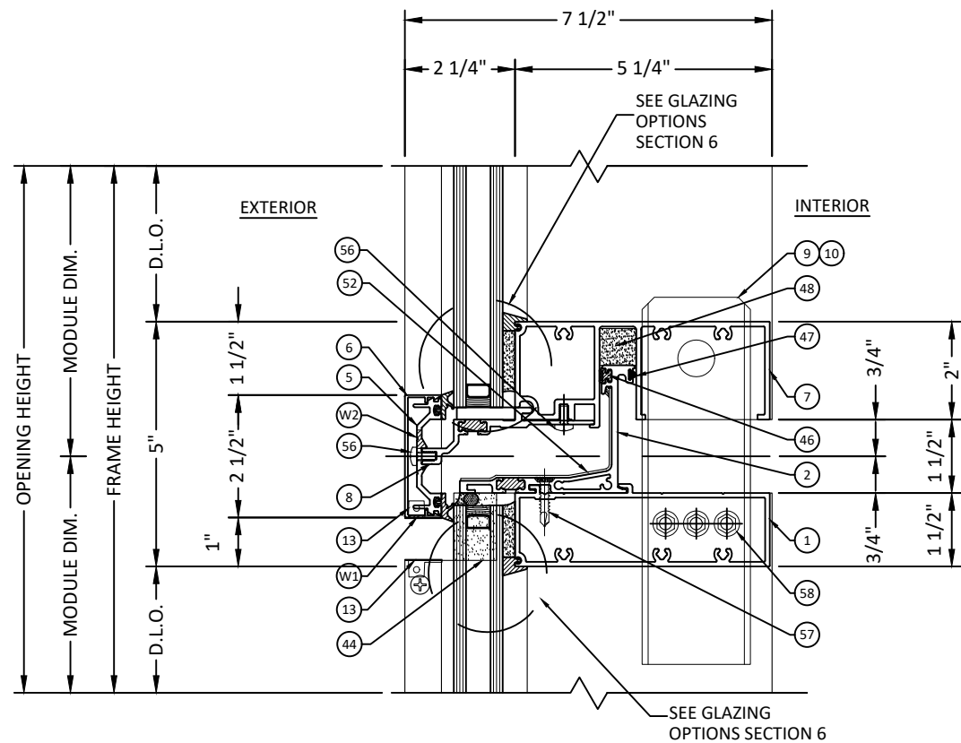
2 3.0 VERTICAL SECTION CAPTURE - STACKING HORIZONTAL
