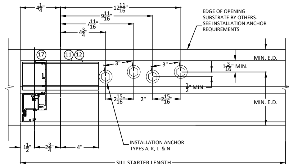
5 HORIZONTAL SECTION 7.3 SILL STARTER AT JAMB CONFIG 2
