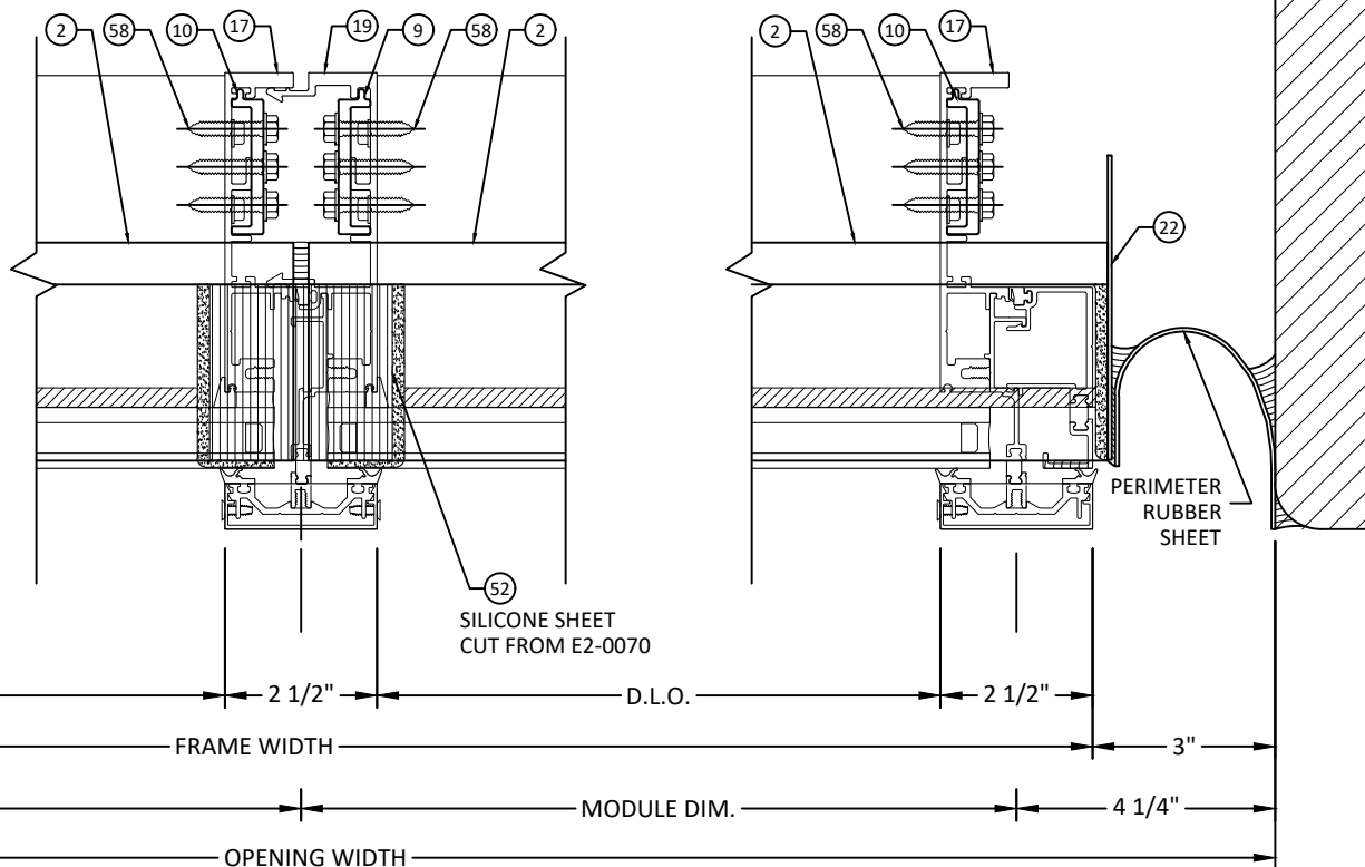
6 HORIZONTAL SECTION 4.0 SPLICE - CAPTURE/SSG
