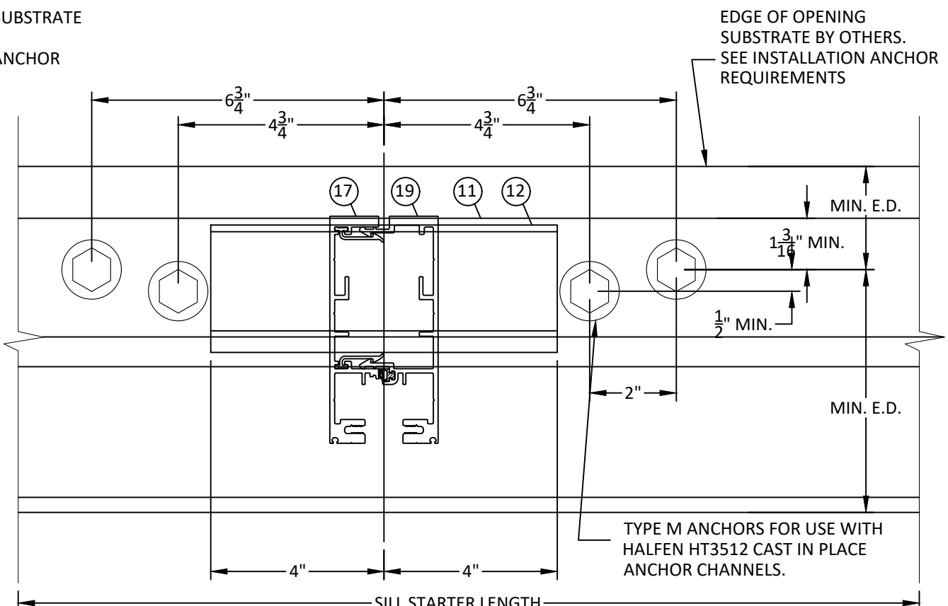
4 HORIZONTAL SECTION 7.2 SILL STATER AT MULLION CONFIG 1
