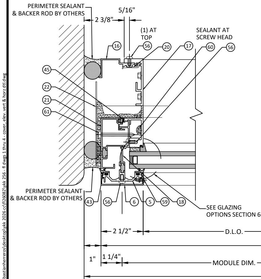
5 HORIZONTAL SECTION 4.0 CAPTURE
