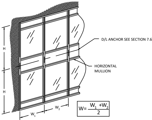
DOUBLE SPAN
